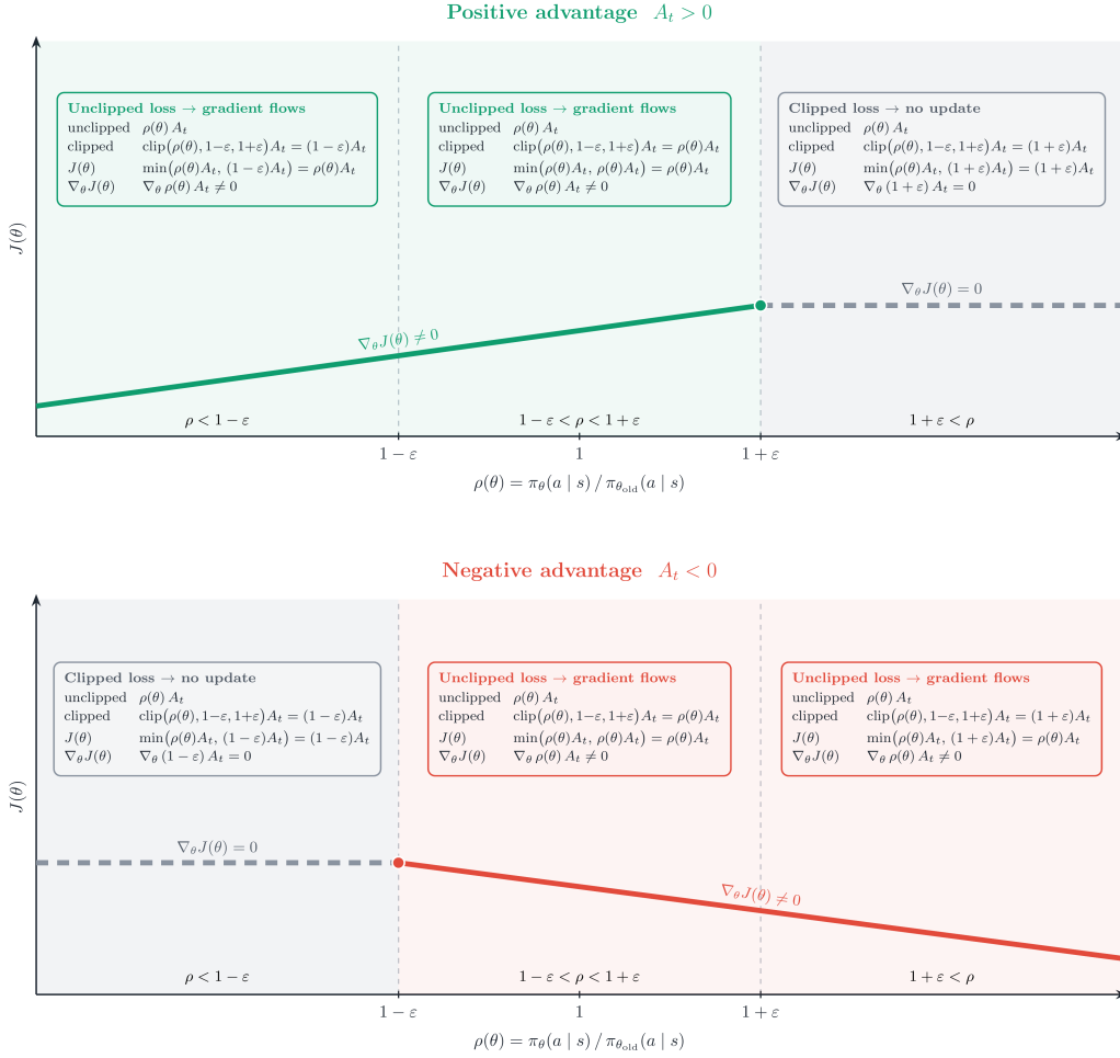
Figure 20: Visualization of the PPO objective J(\theta) as a function of the policy ratio \rho(\theta) , for both positive and negative advantage. Within each panel, the three ratio regions are annotated with their unclipped term, clipped term, resulting objective, and gradient.
