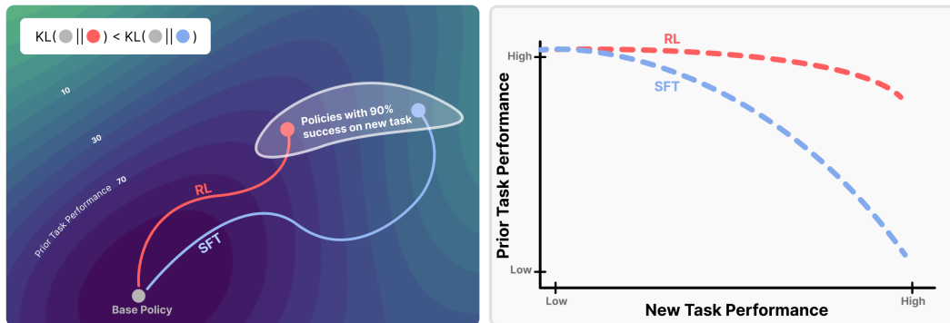
Figure 44: Bias toward KL-minimal solutions reduces forgetting. (Left) Among policies that solve the new task, RL converges to those closest in KL to the base model. (Right) This KL bias yields higher prior-task retention at matched new-task performance compared to SFT. From Shenfeld, Pari, and Agrawal 2026. License CC-BY.
