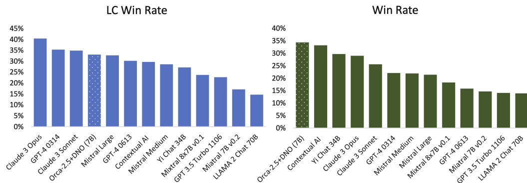
Figure 48: Results from the paper on Direct Nash Optimization (DNO) highlighting their small model outperforming the likes of GPT-4. Rosset et al. 2024. License CC-BY.
