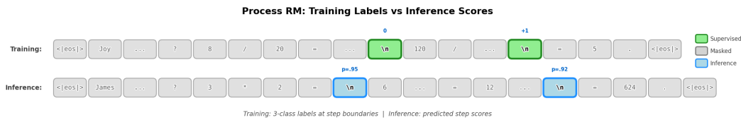
Figure 15: Process reward models provide supervision only at step boundaries (e.g., newline tokens). Each step receives a 3-class label: correct (+1), neutral (0), or incorrect (-1). All other tokens are masked during training.
